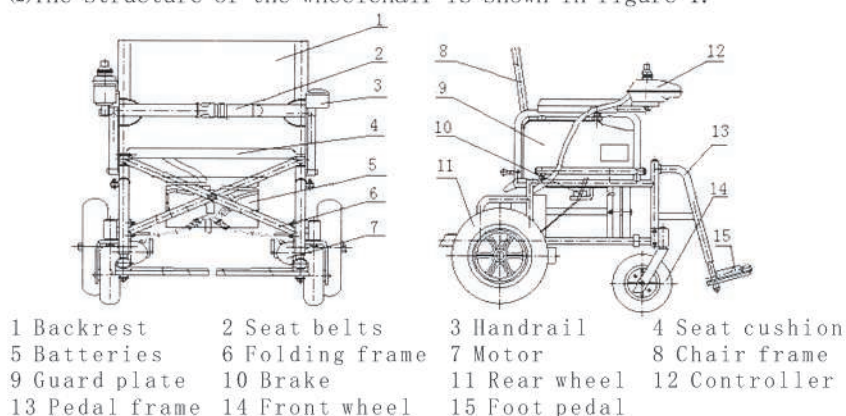
Fig. 1 schematic diagram of electric wheelchair structure
